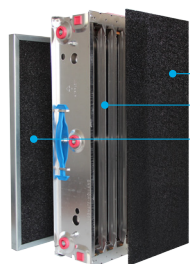
Filter construction: • Pre-filter • ElectroMax filter • Activated carbon filter
